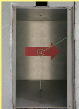
Position of the thermal links or thermal bulbs mechanisms in the air stream for threshold temperature limit measurement
